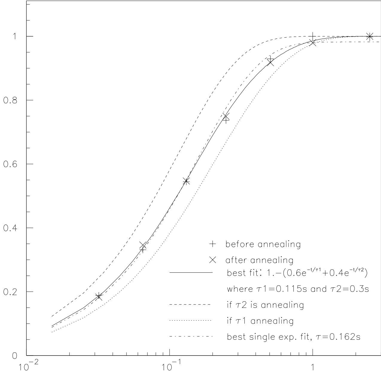
Relative traps capacity vs. time since sweeping charge injection (sec)
